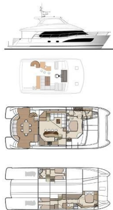
PC60 Layout
