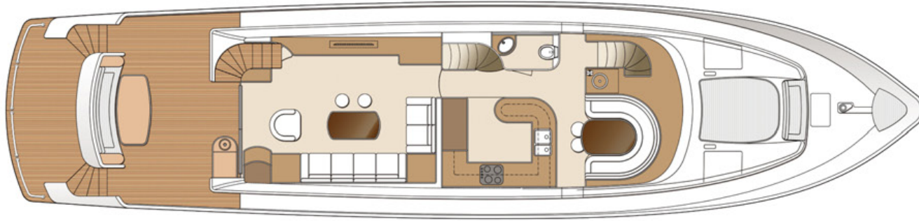
MAIN DECK
