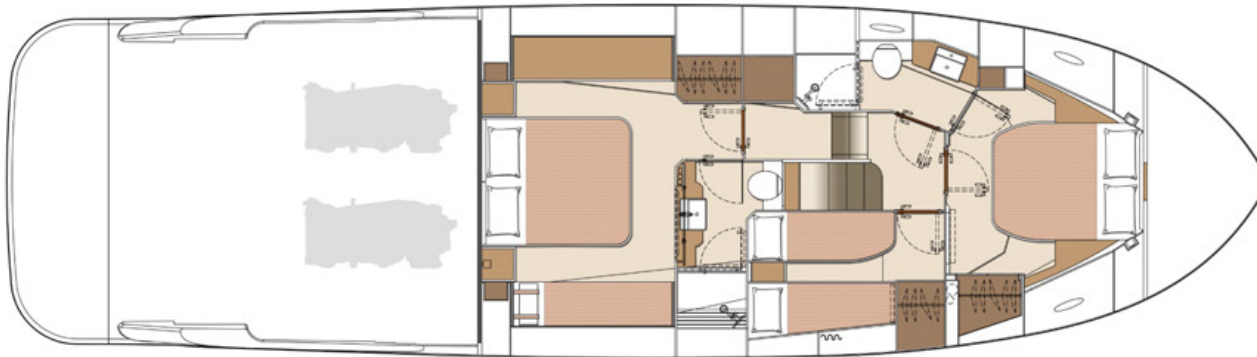
LOWER DECK
