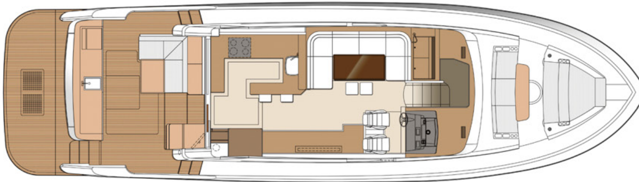
MAIN DECK
