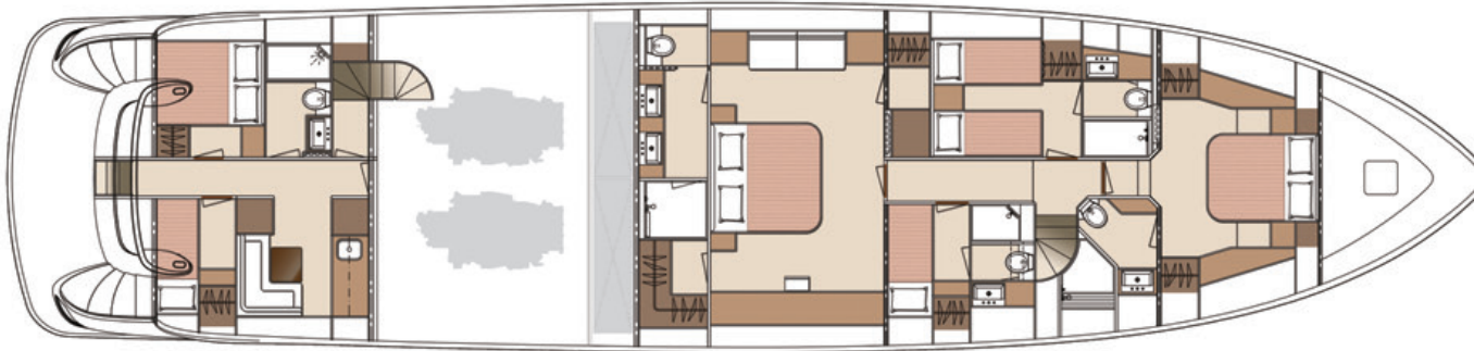
LOWER DECK
