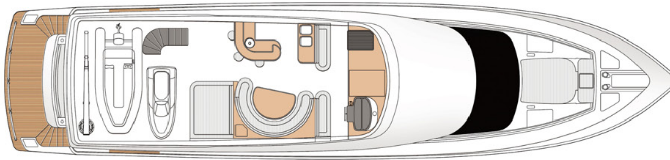
UPPER DECK
