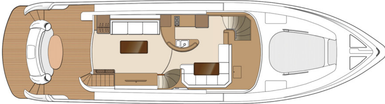
MAIN DECK
