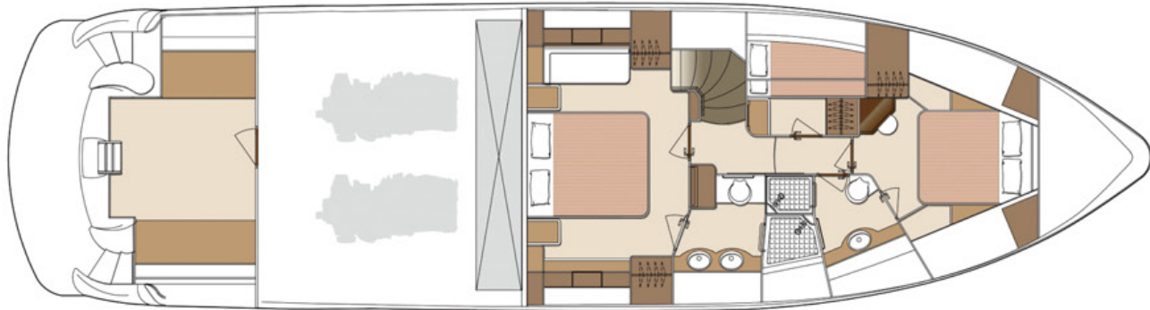
LOWER DECK
